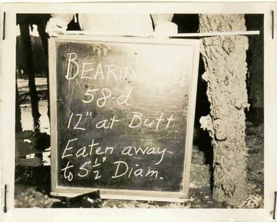
Neg. No DB 7699 Dispo: L HQ Dest Photo'g Ellis Dept MCE & M Caption CONDITION OF JETTY AT HMCS "CORN- WALLIS".
